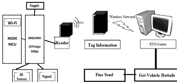
Fig 2. System architecture
